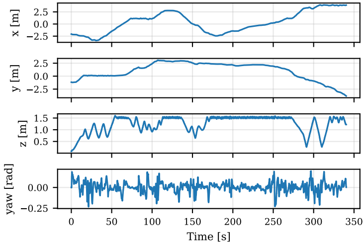
exp 1 - UAV 0 - Position
